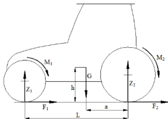
Diagram of forces and moments acting on a 4x4 tractor - braking applied on all wheels
